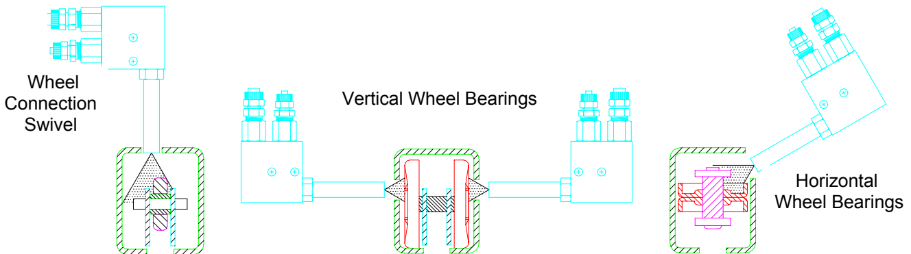
Overhead Power Chain Conveyor - Enclosed Track Four Nozzle Continuous Spray
